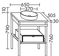
MYA #29 Ceramic washbasin with vanity unit
