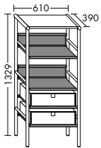
MYA #23 Shelving unit with drawers
