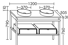
MYA #31 Ceramic washbasin with vanity unit
