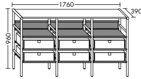
MYA #26 Sideboard with drawers
