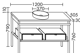
MYA #30 Ceramic washbasin with vanity unit
